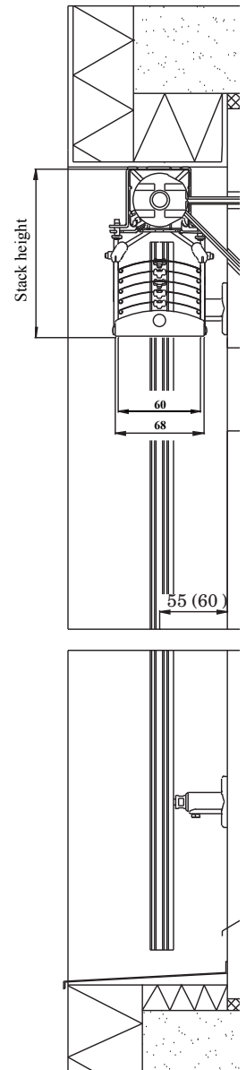
Bottom fix bracket for cable guiding
