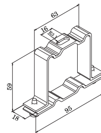
Standard head-box mount bracket
