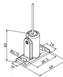
Bottom fix bracket for cable guiding
